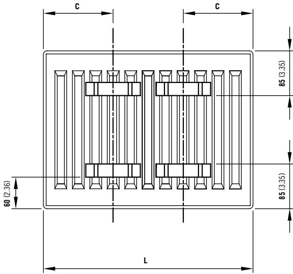
REAR ELEVATION
